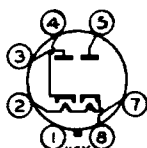
BOTTOM VIEW (G-7Q)
